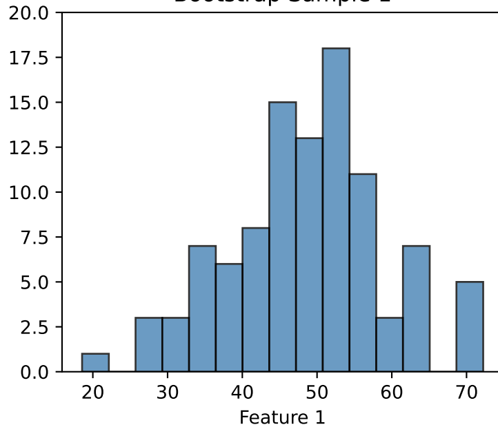
Bootstrap Sample 1
