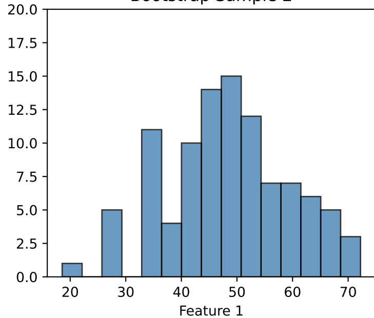
Bootstrap Sample 2
