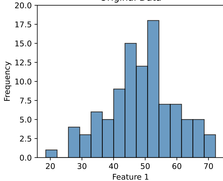
Original Data
